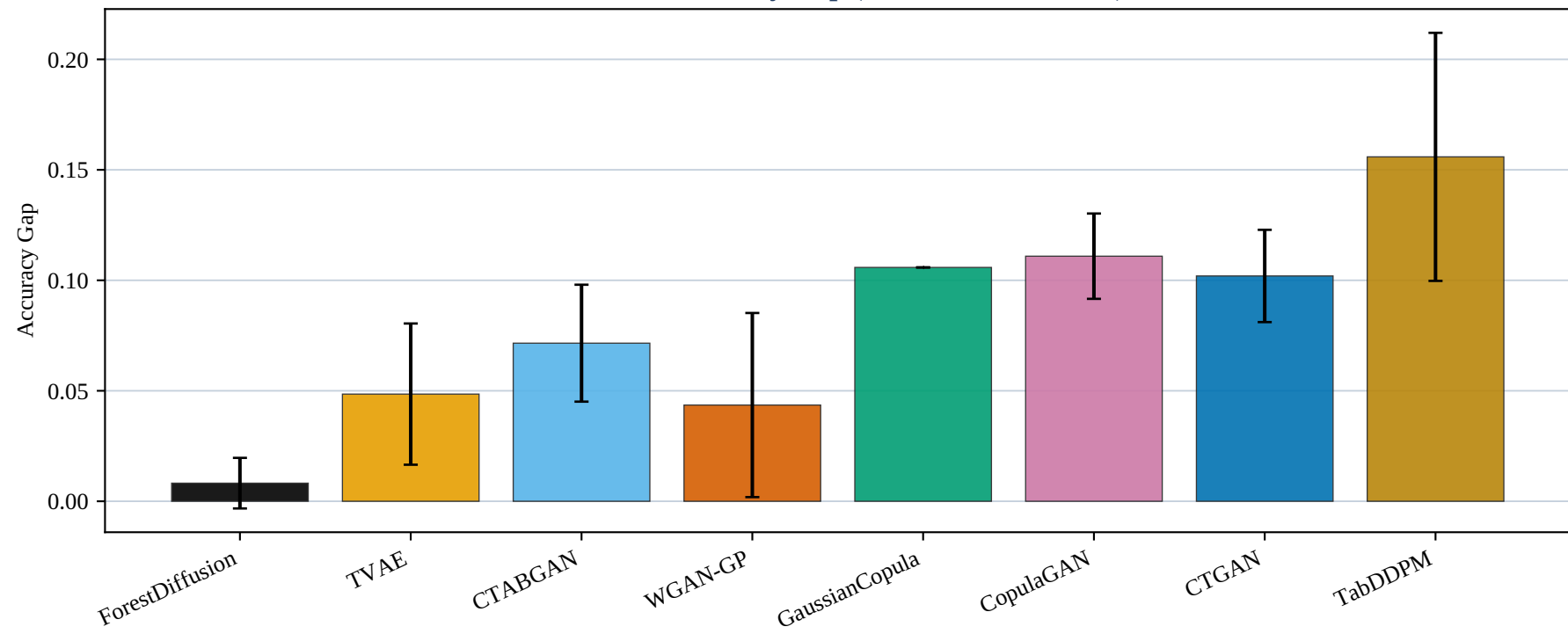
Adult — Accuracy Gap (mean \pm SD, 10 seeds)
